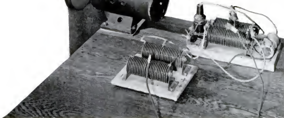
Electroplating setup consists of small transformer and the full-wave rectifier diagrammed in Fig. 9. Four disks are stacked on an insulated bolt. The resistor at right in the photo adjusts current to suit various sizes of work.
